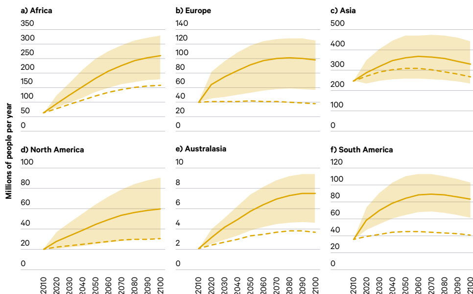
Figure 15. Populations experiencing a drought of at least six months with 12-month accumulated Standardized Runoff Index of less than -1.5, by continent
